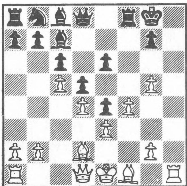
242 After 13 hxg5
